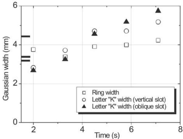
Fig. 12. Gaussian width vs. time for the stripes in the THz image formed with “K and ring” aperture (see Fig. 11) and recorded with the TOD technique. Width profiles were plotted for the trace marked with white line in Fig. 9. The geometrical widths of the slots are shown at the abscissa axis. Some points at the beginning of the curves have very high dispersion due to small noise/signal ratio originated from the speckle effect.
