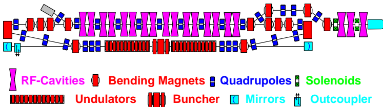
Fig. 2. Scheme of the existing accelerator-recuperator based terahertz FEL.
