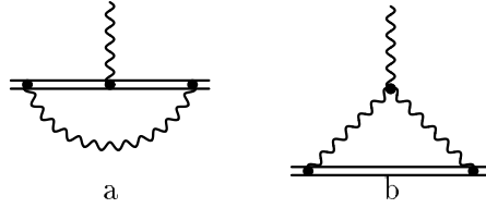
Figure 2: One-loop vertex diagrams
