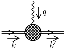
Figure 1: HQET quark-gluon vertex
