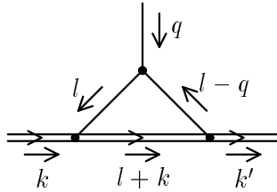
Figure 8: Feynman integral V
