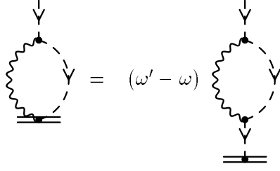
Figure 5: Non-standard vertices
